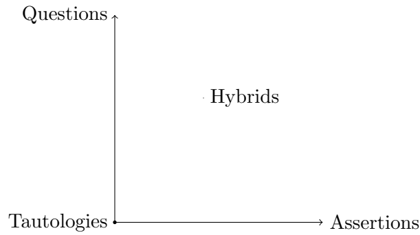
Figure 4. Questions, assertions, hybrids, and tautologies in a two-dimensional space.
