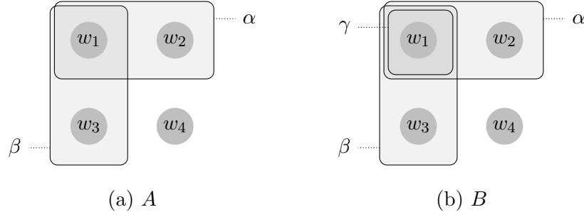
Figure 2. Two non-identical propositions that are equivalent w.r.t. \models .
