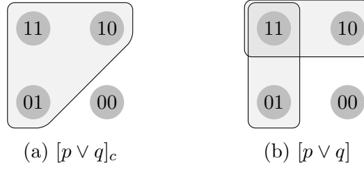
Figure 3. The proposition expressed by p \vee q , classically and in \text{Inq}_{\mathbb{B}} .
