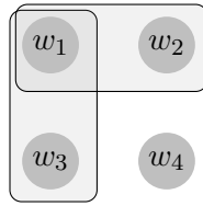
Figure 1. Capturing informative and inquisitive content using sets of possibilities.
